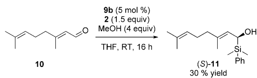
Scheme 2. Copper-catalyzed silyl 1,2-addition to citral 10 .
